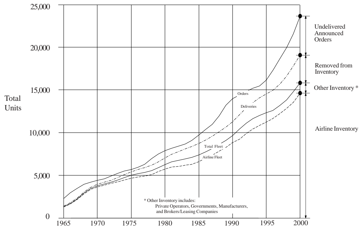
Chart 4 - World Airplane Fleet Status
