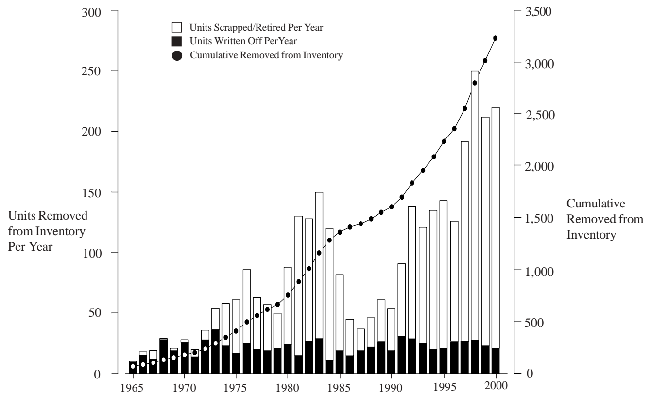
Chart 4 - World Airplane Fleet Status
